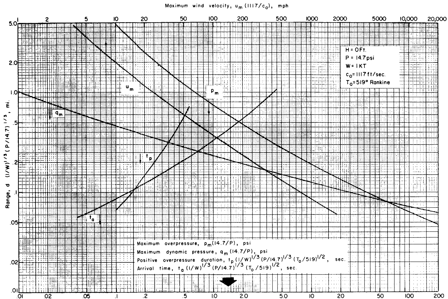
Fig. 2.1—Scaled blast parameters for surface bursts as a function of scaled range. These are plots of Eqs. 2.4, 2.6, 2.8, 2.12, and 2.16 given in Table 2.1. The four effects parameters listed at the bottom of the chart and the one at the top are read on the lower and upper scales, respectively.
